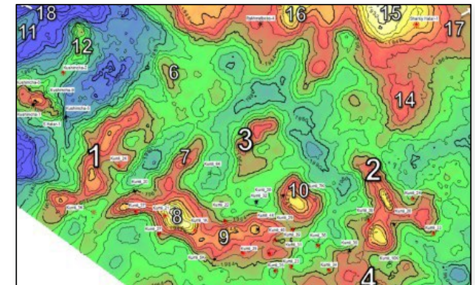
Kumli field: 30 identified 18 target structures
