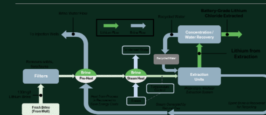
Direct Lithium Extraction (DLE) brine processing
